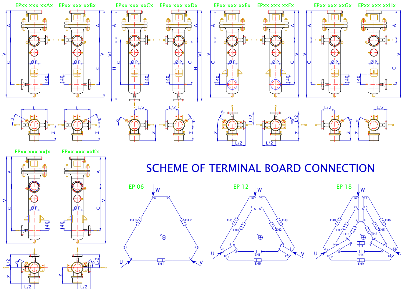
Dimensions of basic type EP 06, EP 12 and EP 18 for pressure PN 63
