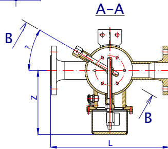
Dimensions of basic type EP 06, EP 12 and EP 18 for pressure PN 40
