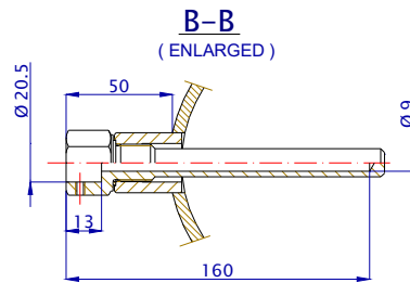
Dimensions of basic type EP 06, EP 12 and EP 18 for pressure PN 40
